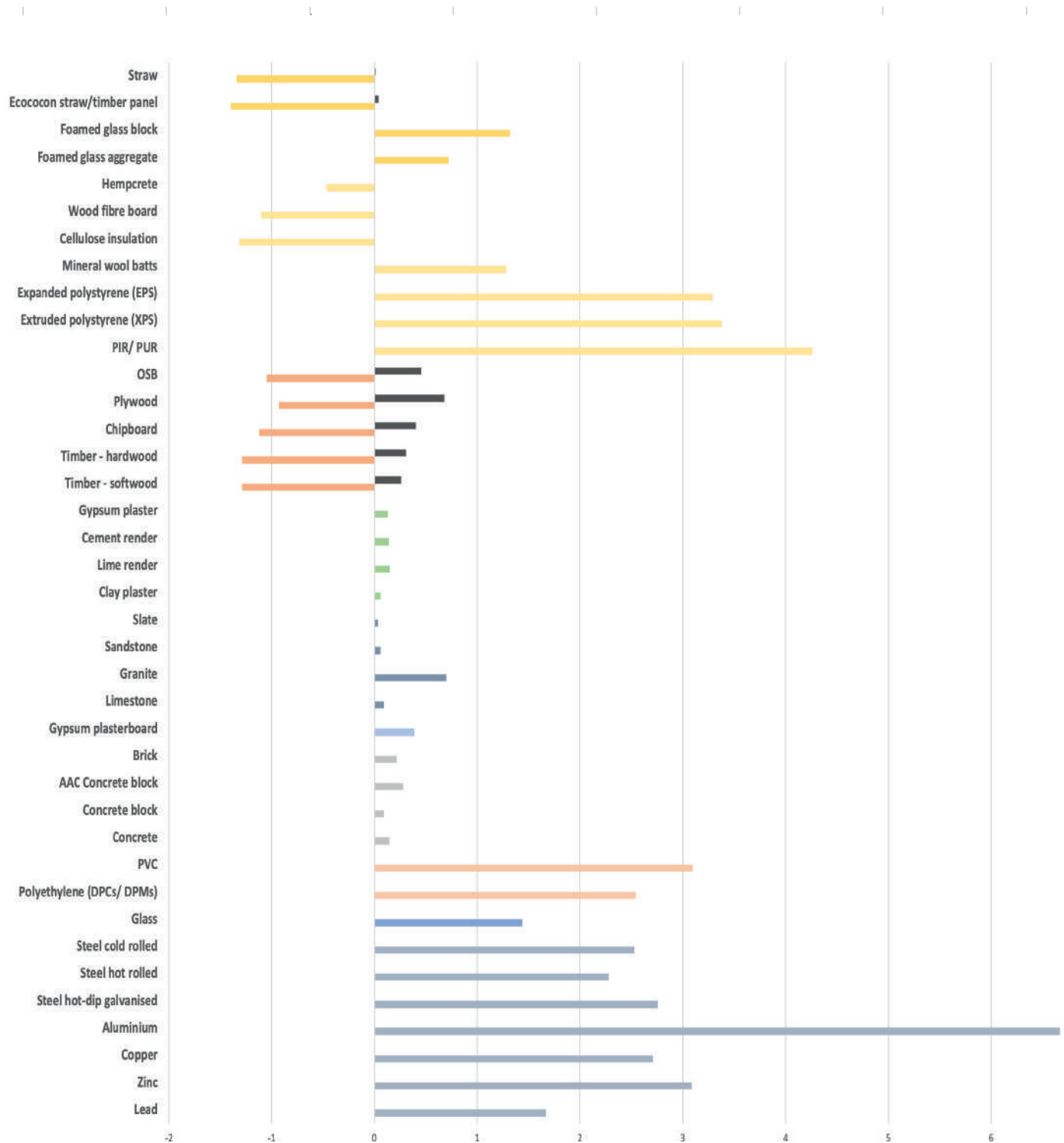
kg CO 2 cradle to gate emissions per kg of material, including sequestration of biobased materials (dark grey - without sequestration)
